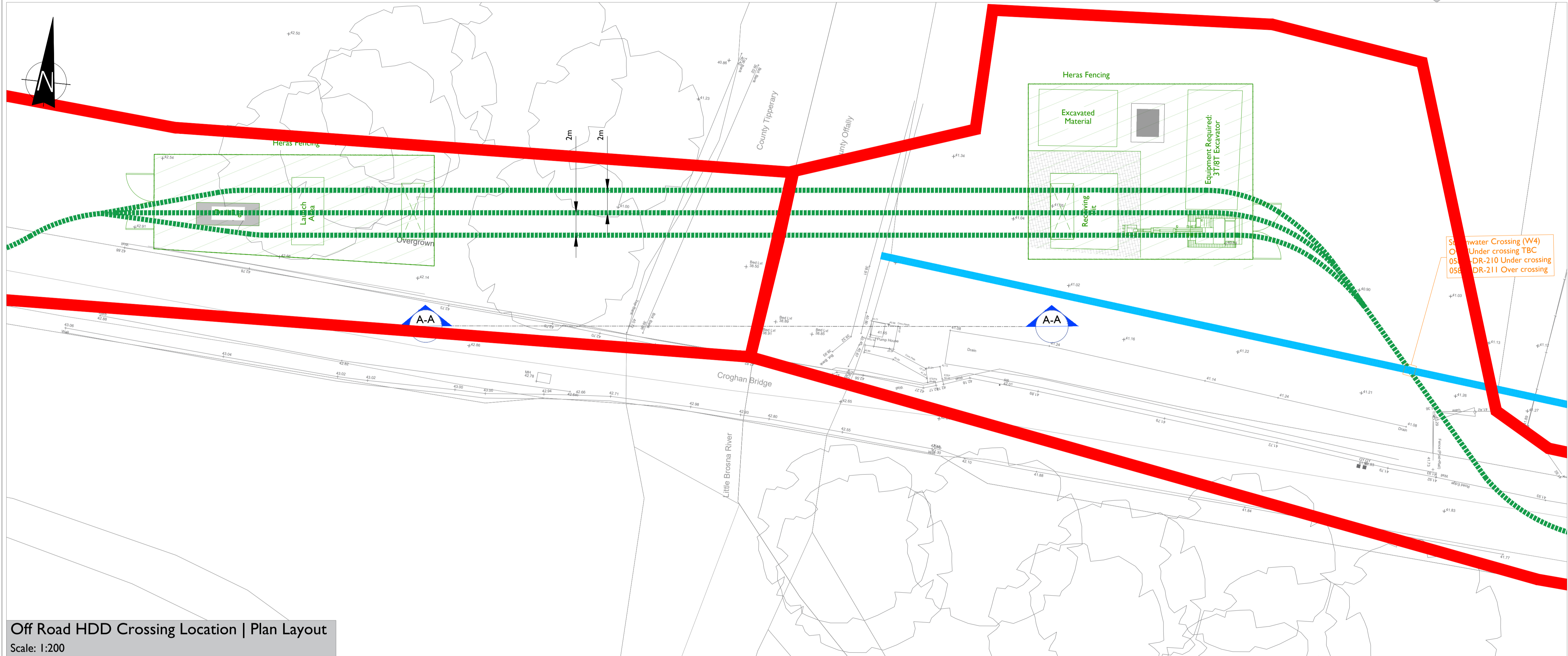
Image 1 | Bridge 2 (W3) To be Avoided by Off Road HDD
