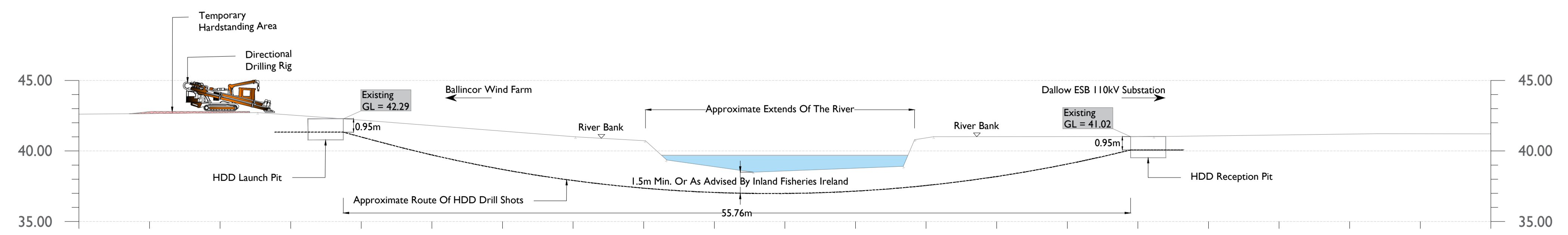
Section A-A | Off Road HDD Under Little Brosna River Scale: 1:200
